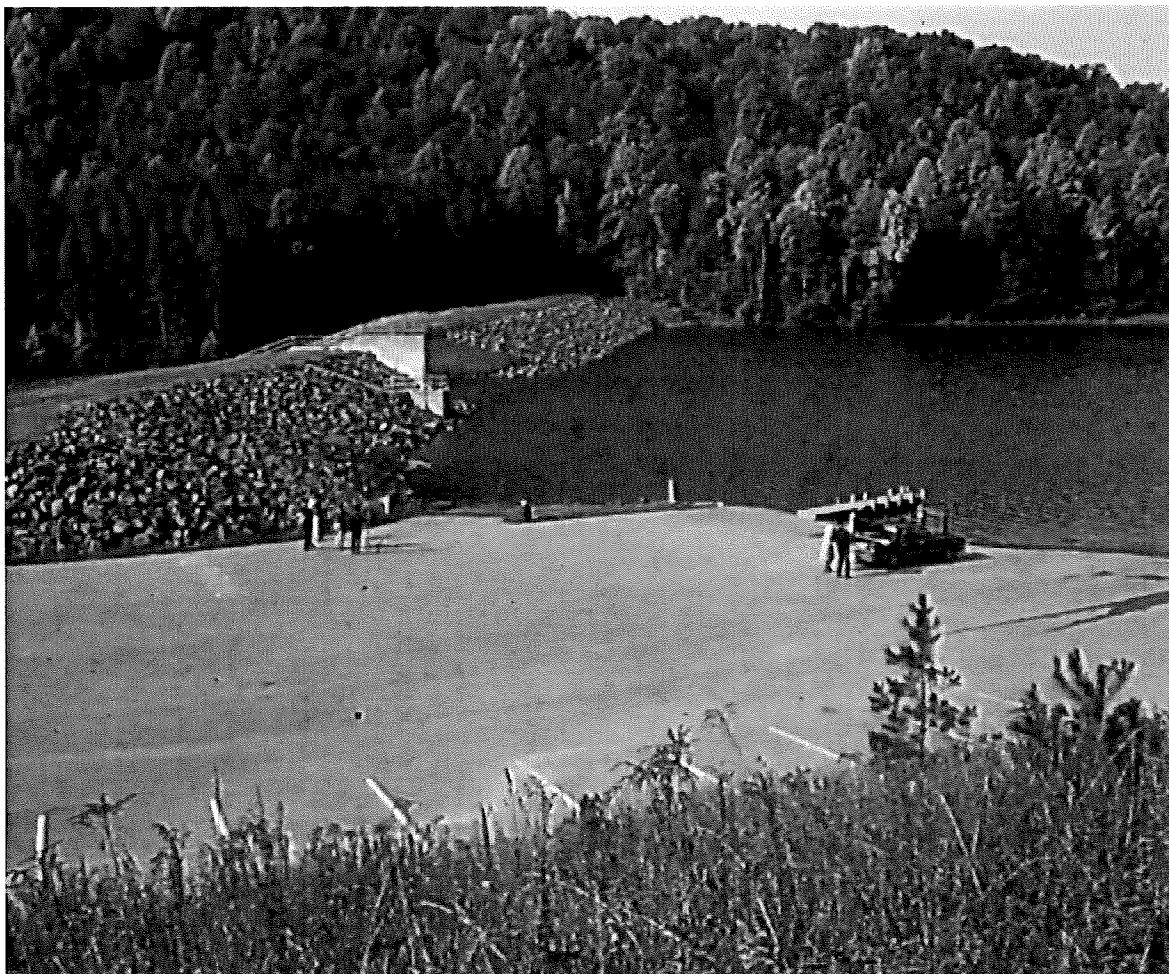
An emergency spillway being used as a parking lot and boat launching ramp.
