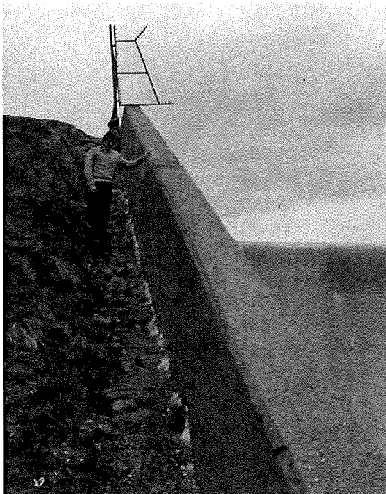
Upper right: Groundhog burrow and undermining of a concrete gutter
