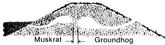
Dangerously close burrows
