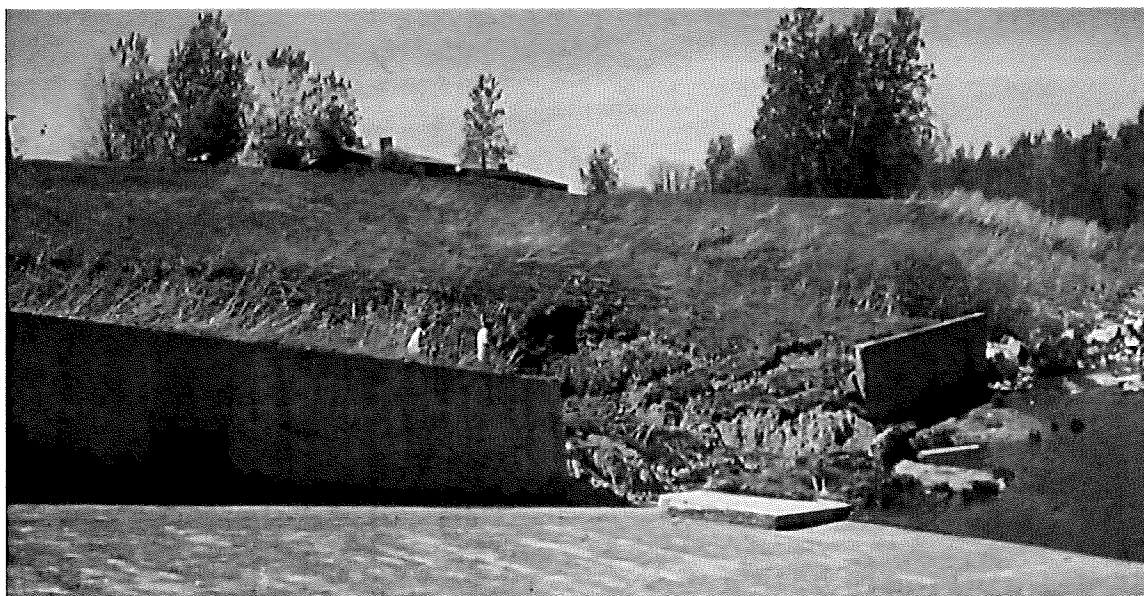
Collapse of spillway wall section.
