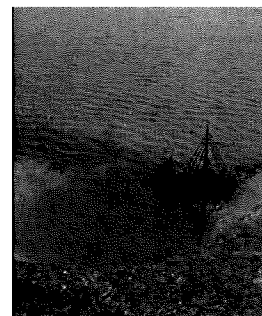
A large sinkhole on the downstream slope and the corresponding sinkhole on the upstream slope at the waterline next to the spillway inlet.
