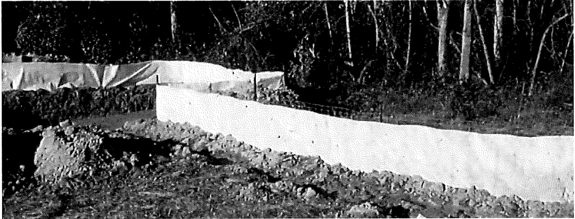
Sediment collected by silt fence used to slow the velocity of flowing water.
